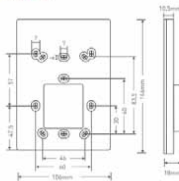
UX8 Touch Panel
