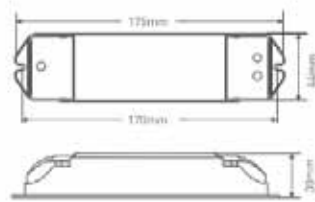
RA-5A/RA-CC Receiver
